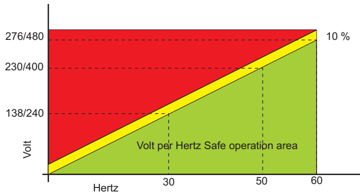
LX Transformer voltages in respect to Frequency
